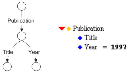
Figure 2: DataGuide constructed over result of finding all publications
