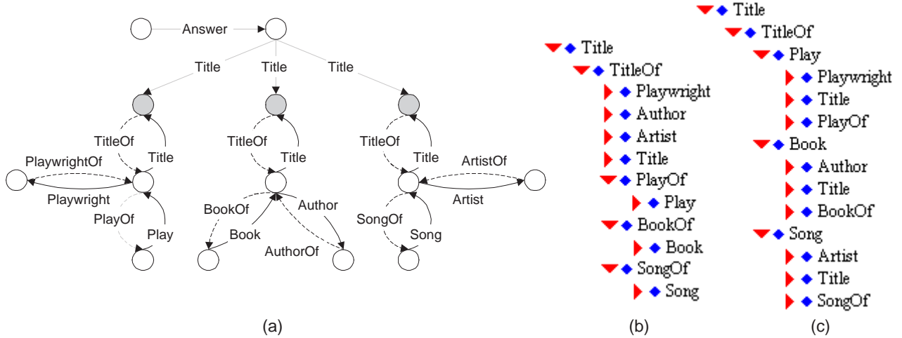
Figure 3: An OEM query result and two potential DataGuides
