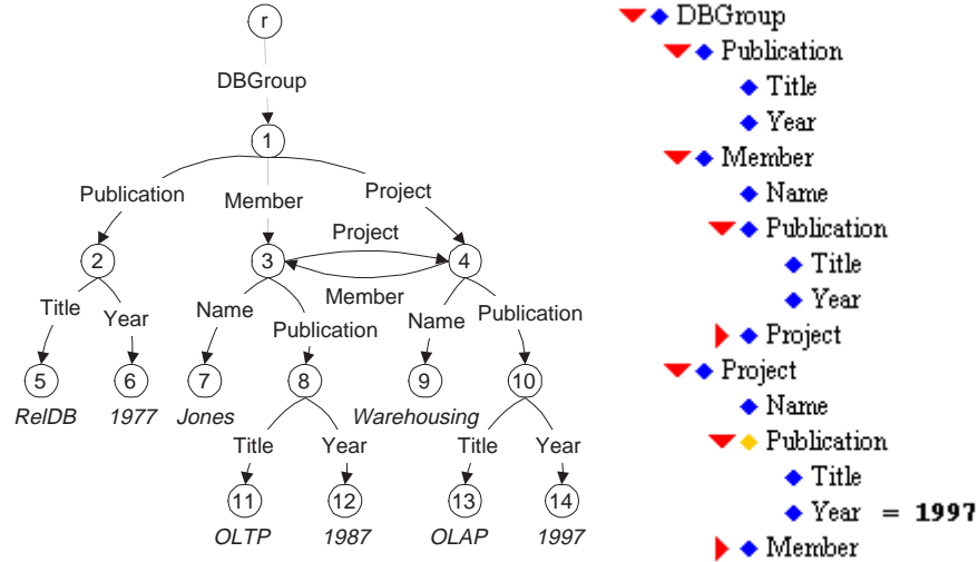
Figure 1: A sample OEM database and its Java DataGuide
