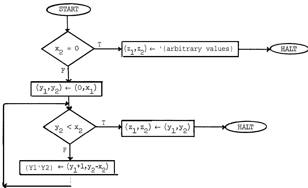
Figure 4: Another division program
