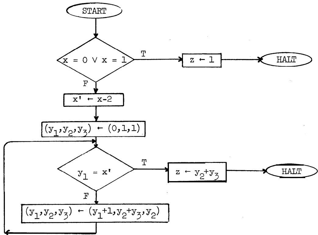
Figure 13: Iterative fibonacci program
