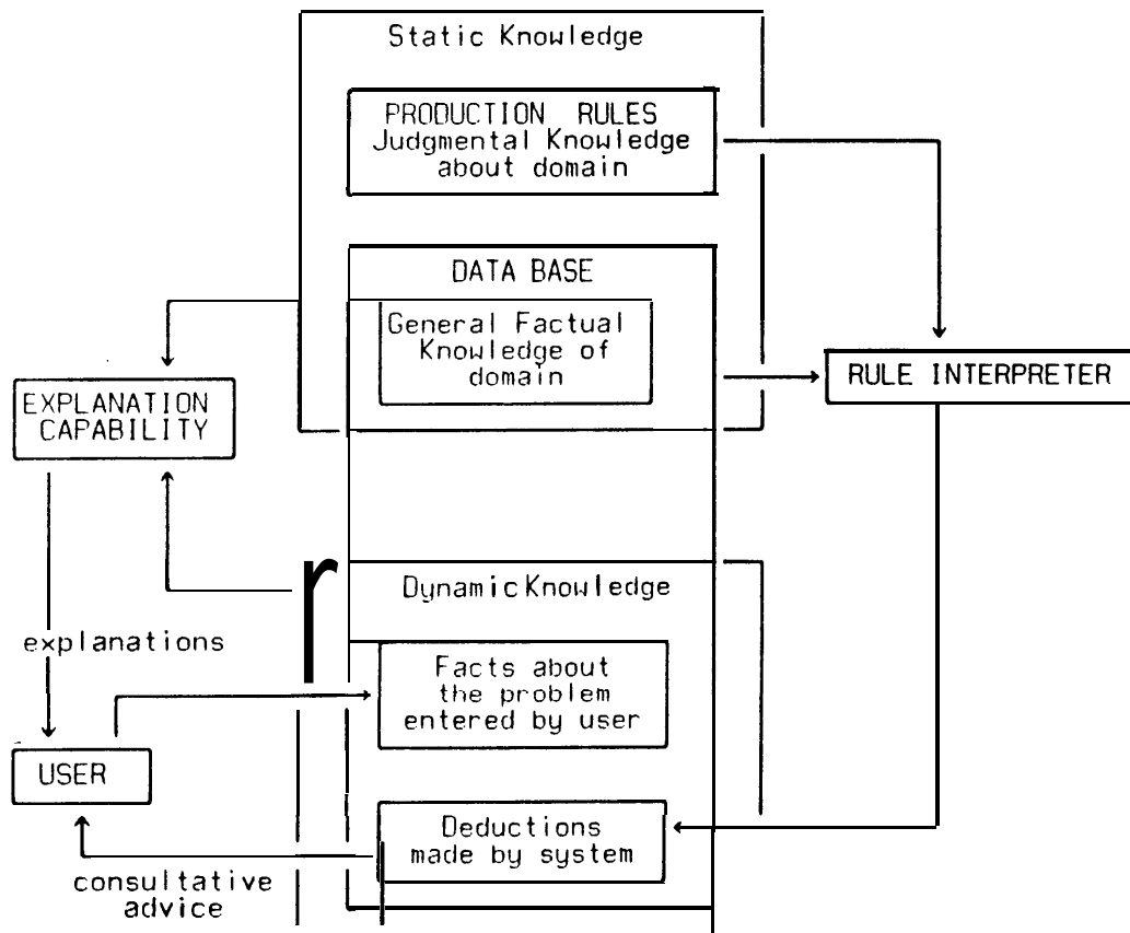
Figure 1. A Production-Based Consultation System with Explanation Capability
