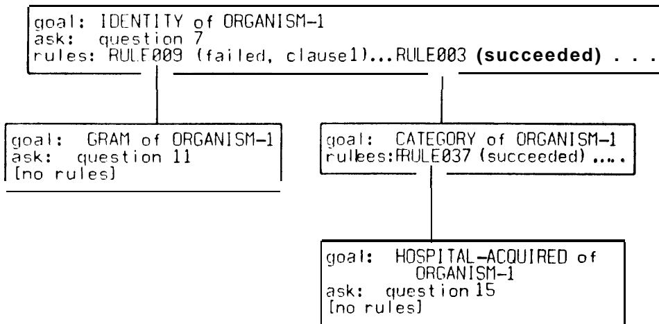
Figure 4. Portion of a History Tree
