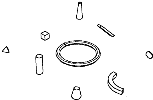
Figure 8. Generalized Cone Examples
