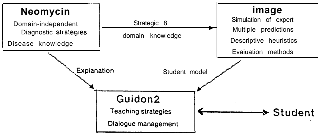
Figure 1-1: Components of the GUIDON2 teaching System
