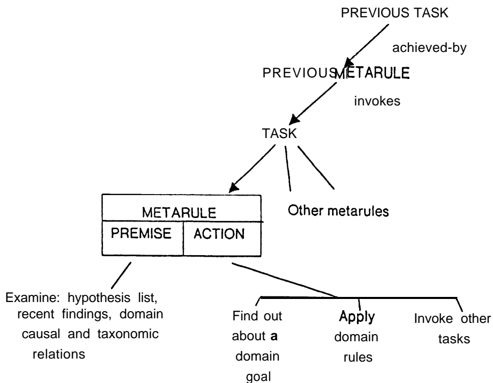
Figure 3-2: Abstraction of a Task and Its Metarules
