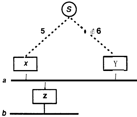
Figure 3: Reverse Path Forwarding Example
