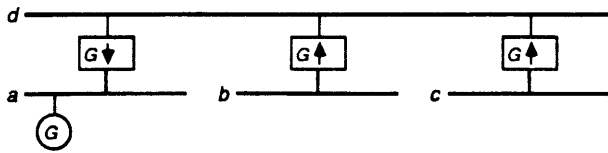
Figure 1: Bridged LAN with One Group Member
