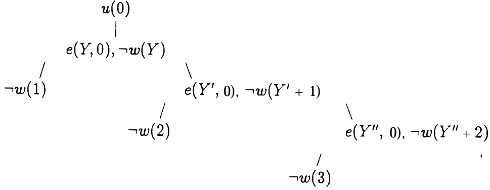
Figure 3: SLP-tree u_0
