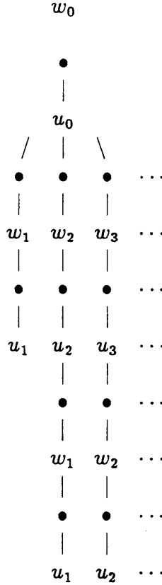
Figure 4: Global tree for \leftarrow w(0) . Each w_i is successful, and each u_i is failed.
