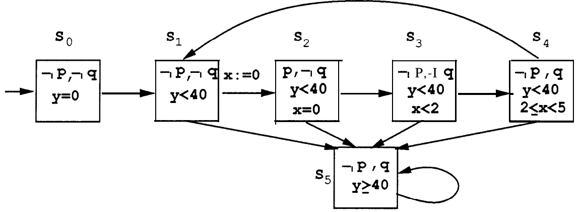
Figure 1: Timed automaton
