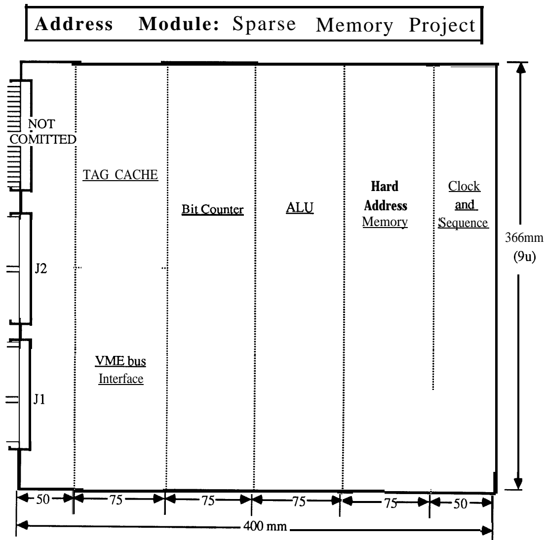
Figure 2.1: Floorplan.
