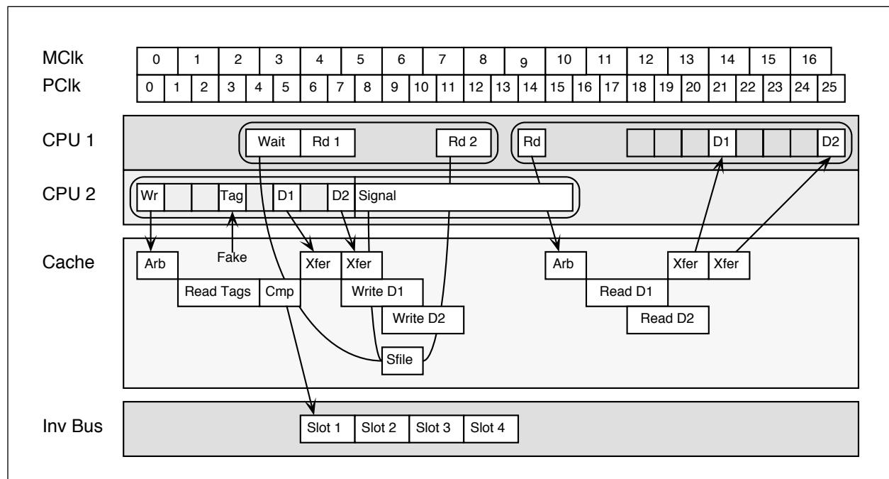
Figure 6. An interprocessor communication example.
