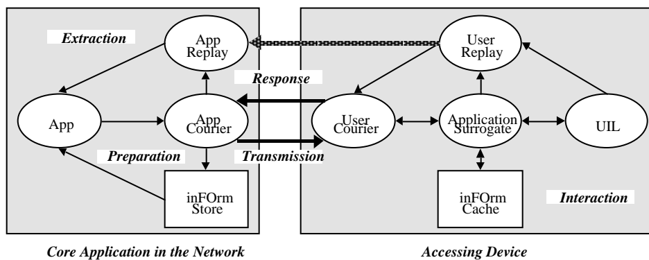
Figure 3.2: DIANA: Overall Architecture
