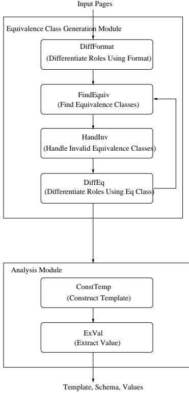
Figure 10: Modules of EXALG
