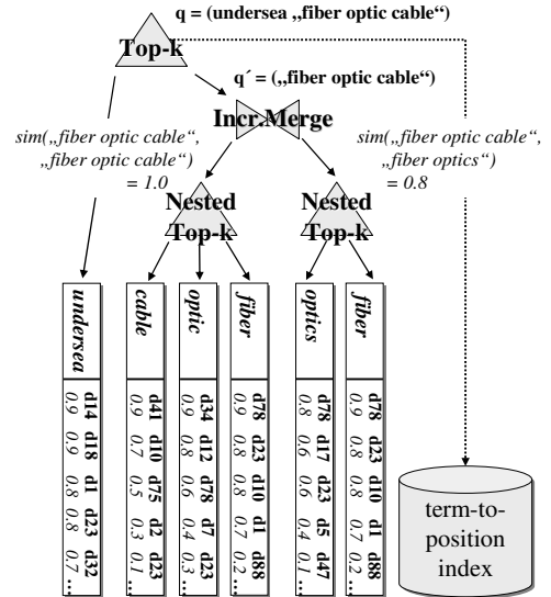
Figure 2: Phrase matching with multiple nested top-k operators
