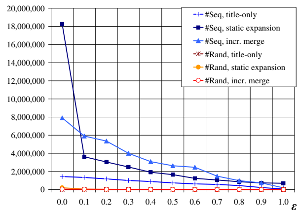
Figure 4: Efficiency as a function of \epsilon
