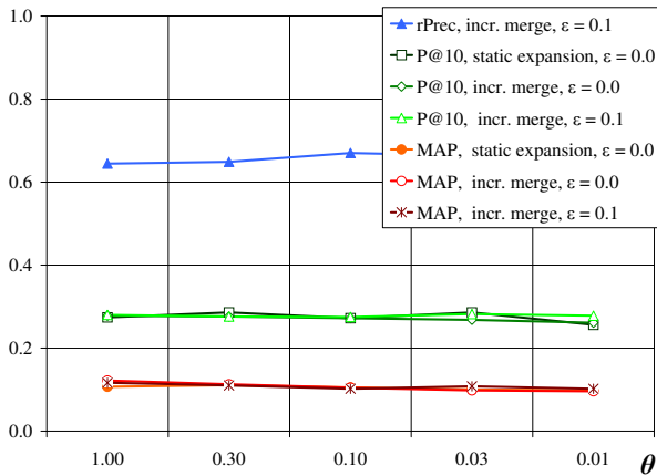
Figure 5: Precision as a function of \theta
