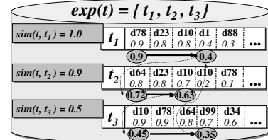
Figure 1: Example schedule for Incremental Merge
