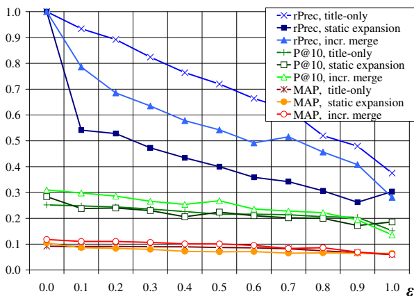
Figure 3: Precision as a function of \epsilon
