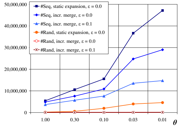
Figure 6: Efficiency as a function of \theta
