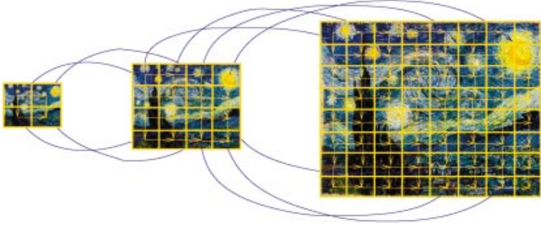
Fig. 6. In the statistical modeling process, spatial relations among image pixels and across image resolutions are both taken into consideration. Arrows, not all drawn, indicate the transition probabilities captured in the statistical model.
